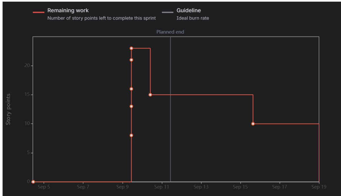
Figure 3 – Burndown Chart
